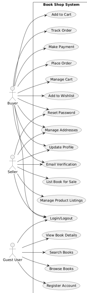
Figure: 1.4 – Use Case Diagram
