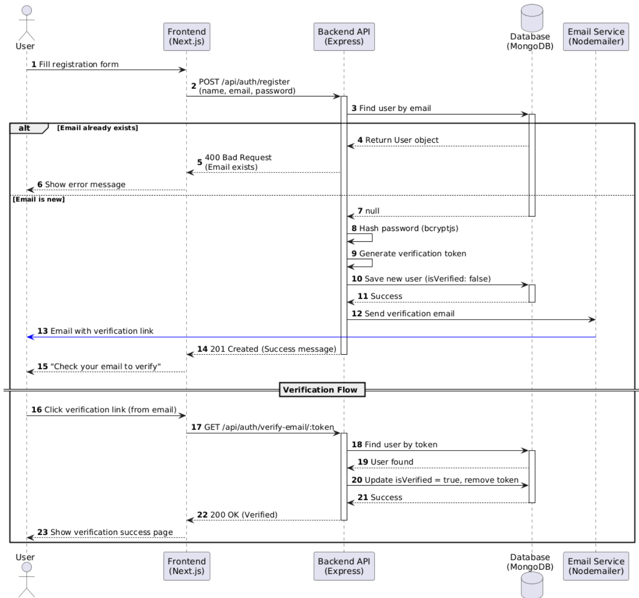
Figure: 1.8 - Sequence Diagram (user registration and email verification)
