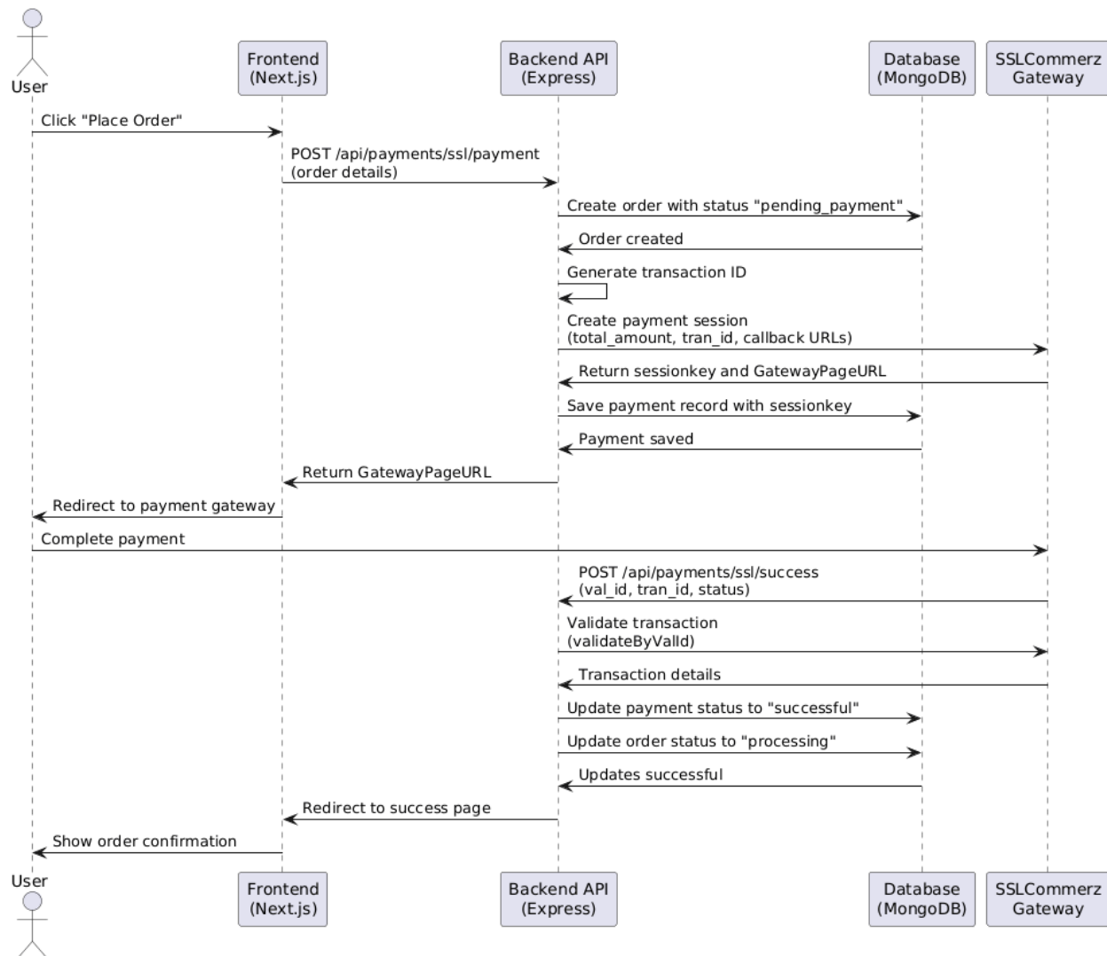
Figure: 1.9 - Sequence Diagram (Payment Processing)
