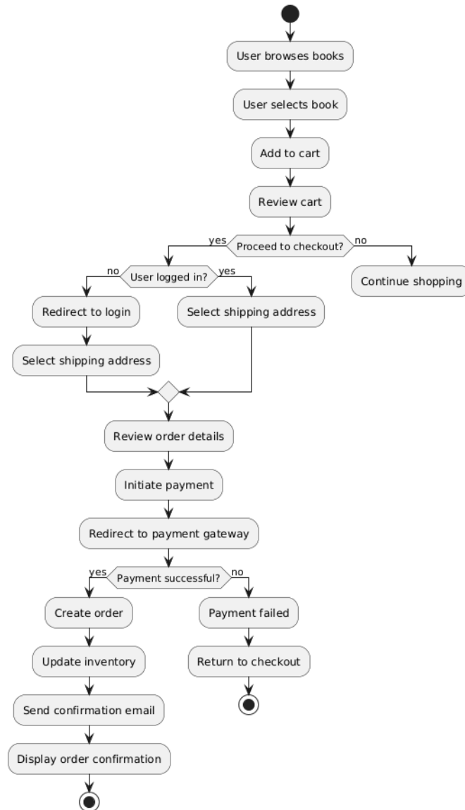
Figure: 1.5 - Activity Diagram (Order Processing)
