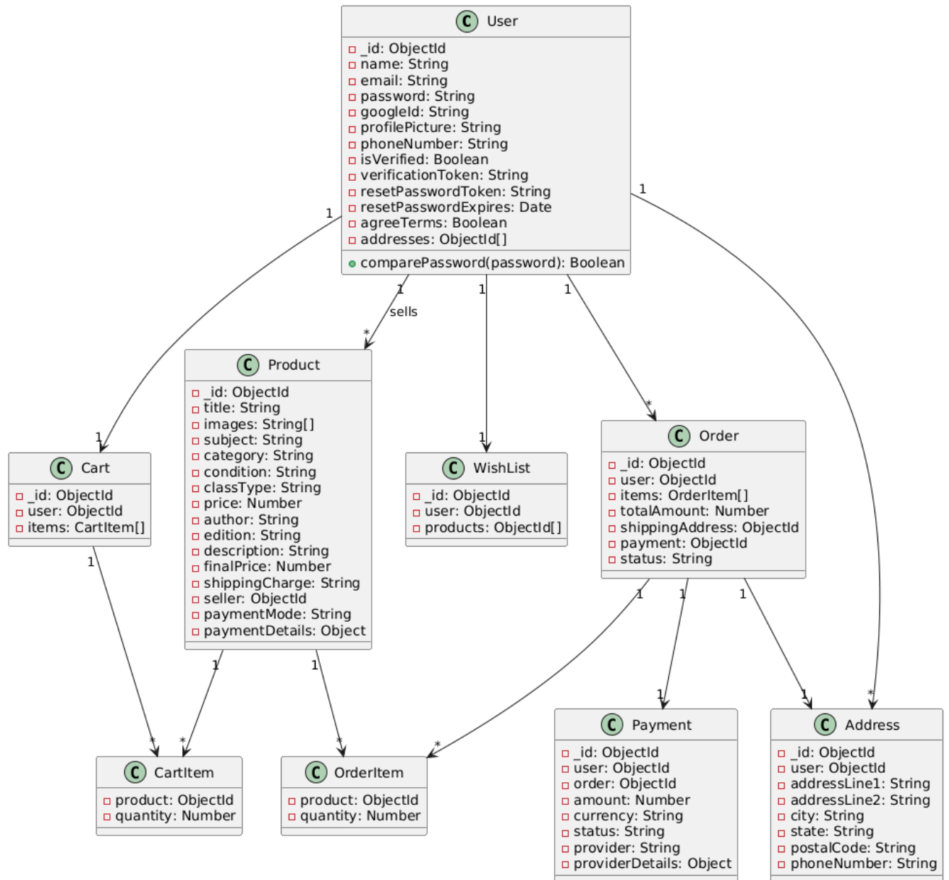
Figure: 1.6 - Class Diagram
