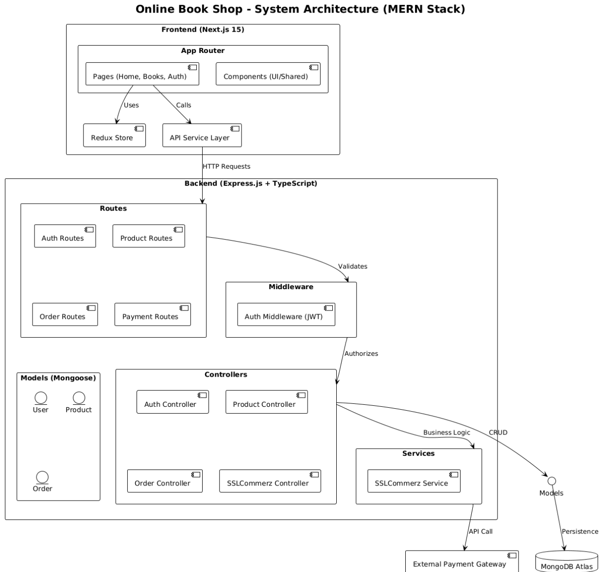
Figure: 1.2 – System Architecture Diagram
